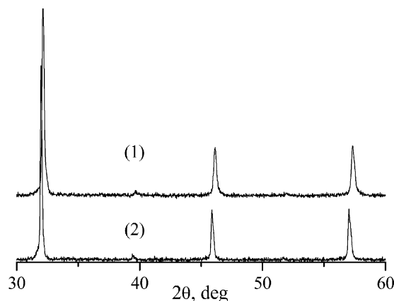
Fig. 2. Diffraction patterns of samples \text{SrCo}_{0.5}\text{Fe}_{0.2}\text{Ta}_{0.3}\text{O}_{3-y} : (1) as prepared, (2) after annealing in vacuum ( P \sim 10^3 Pa) at 950^\circ\text{C} and quenching.
